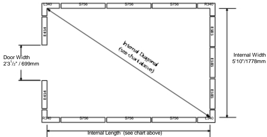
Diagram based on the 6'5" x 8' model
